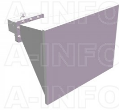
LB-510-15-C-7/16FSPO Standard Gain Horn Antenna 1.45-2.2GHz 15dB Gain 7/16(DIN) Female
