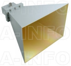
LB-510-15-C-7/16F Standard Gain Horn Antenna 1.45-2.2GHz 15dB Gain 7/16(DIN) Female
